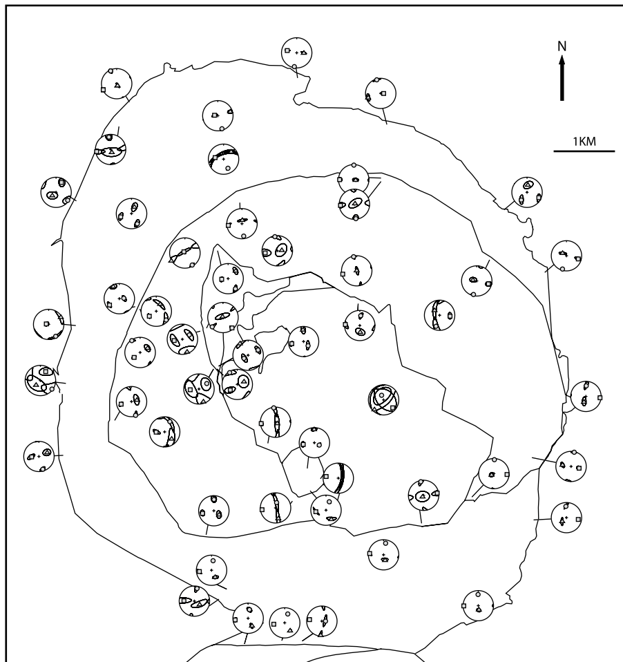
Fig. 16. Stereographic plot of AMS orientation data for the main Rosses Pluton. The margins of the internal units of the pluton are shown in outline and all other lithologies omitted for clarity. Symbols are as in Fig. 12.
