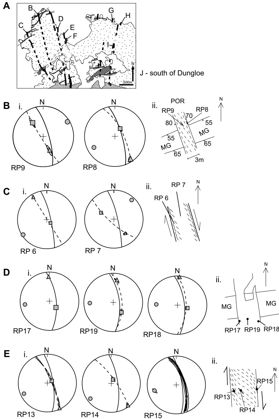
Fig. 17. AMS data for the porphyry dykes. (A) Sketch map showing the location of sample stations. (B–J) i. stereographic plot of AMS orientation data, symbols as in Fig. 12 plus solid great circles – dyke margin, dashed great circles – AMS foliation; and ii. sketch showing the interpretation of sense of shear.
