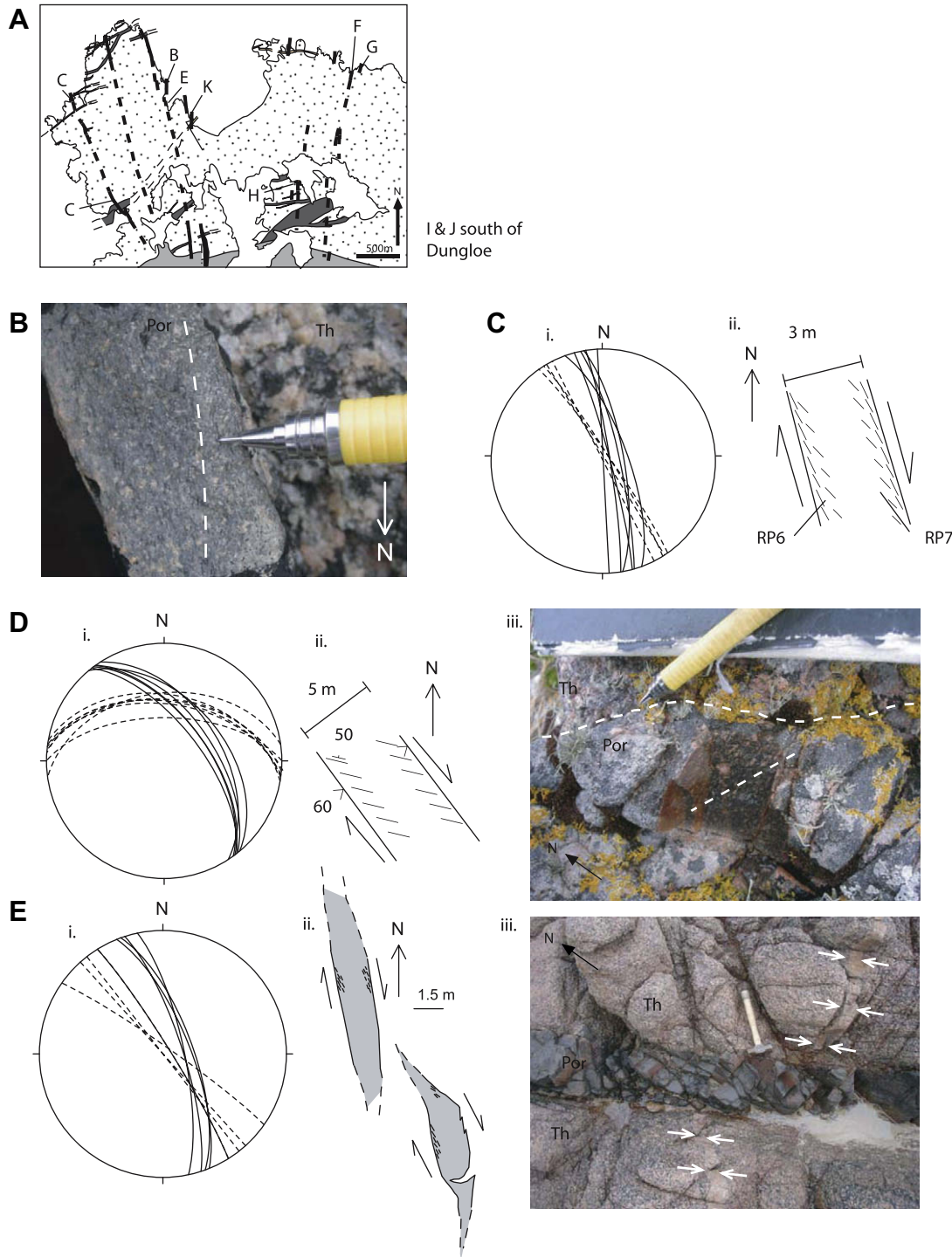
Fig. 9. Visible fabric data from the porphyry dykes. (A) Sketch map showing the locations of where fabrics were measured in parts B–H. (B) Field photograph of the margin of a porphyry dyke. A fabric defined mainly by biotite (highlighted with a dashed white line) is observed at an apparent low angle to the margin between the porphyry (Por) and Thorr granodiorite (Th). (C) i. Stereographic projection of contacts (solid lines) and visible fabrics (dashed lines) measured at this locality; and ii. sketch map of the fabric–contact relationships indicating a dextral sense of shear. (D and E) i. Stereographic projection of contacts (solid lines) and visible fabrics (dashed lines) measured at this locality; and ii. sketch map of the fabric–contact relationships indicating a dextral sense of shear; and iii. field photograph displaying these fabric–contact relationships. (F–I) i. Stereographic projection of contacts (solid lines) and visible fabrics (dashed lines) measured at this locality; and ii. sketch map of the fabric–contact relationships indicating a dextral sense of shear. (J) Stereographic projection of contacts (solid lines) and visible fabrics (dashed lines) measured at this locality. (K) Field photograph showing xenoliths of Thorr granodiorite displaying lobate contacts. This is the only locality in which these have been found.
