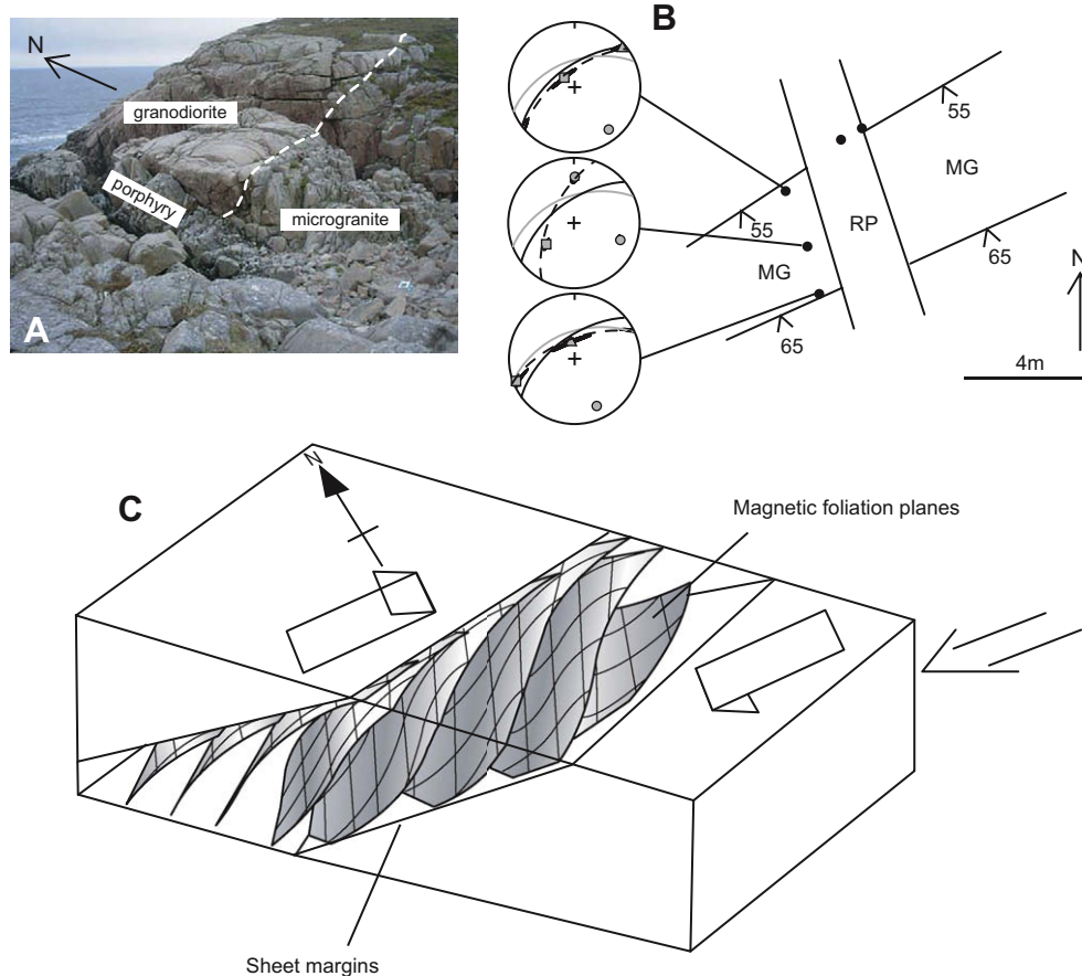
Fig. 12. (A) Field photograph showing the relationship between Thorrs granodiorite, a microgranite sheet and a porphyry dyke. (B) Sketch map of the locality, dip of microgranite (mg) contacts is shown. AMS sample points are indicated and orientation data from these samples plotted stereographically; K_1 axis – square, K_2 axis – triangle and K_3 – circle. Also plotted on the stereonets are great circles for the contacts: upper contact – solid black line, lower contact – solid grey line, and magnetic foliation – broken line. (C) 3D visualisation of the fabric geometry in the microgranite sheet displaying how the AMS foliation is subparallel to the contacts but strikes anticlockwise in the centre.
