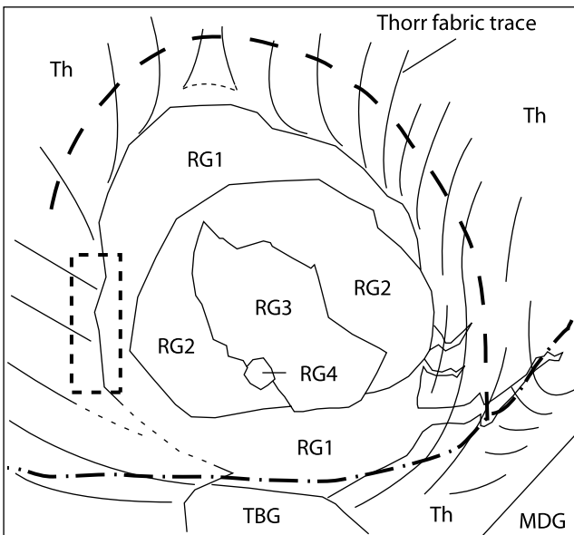
Fig. 3. Summary of the fabric trends in the Thorr Pluton and the contacts of the Rosses Pluton. The limit of deflection of Thorr fabrics close to the Rosses Pluton is highlighted with a dashed line. The limit of deflection of fabrics in the Main Donegal shear zone is highlighted with a dashed and dotted line. The latter may involve a combination of both of these strain fields and results in a tricuspid interference pattern in the southeast of the figure. Only in a small area along the western contact of the Rosses Pluton (highlighted with a dashed box) are Thorr fabrics truncated at a high angle in a similar way to the Trawenagh Bay Granite western contact to the south. Th – Thorr Pluton; TBG – Trawenagh Bay Granite; MDG – Main Donegal Granite, RG1, 2, etc. – Rosses Granite G1, G2, etc.
