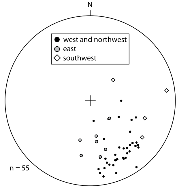
Fig. 4. Stereographic projection showing the orientation of the microgranite sheets in the three main areas.
