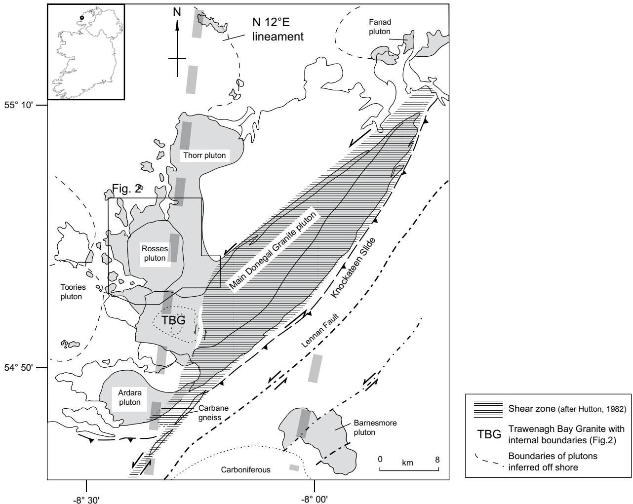
Fig. 1. The plutons of the Donegal Batholith modified after Pitcher and Berger (1972). The extent of the Main Donegal Granite shear zone is taken from Hutton (1982) and the position of the N12°E from Hutton and Alsop (1996).
