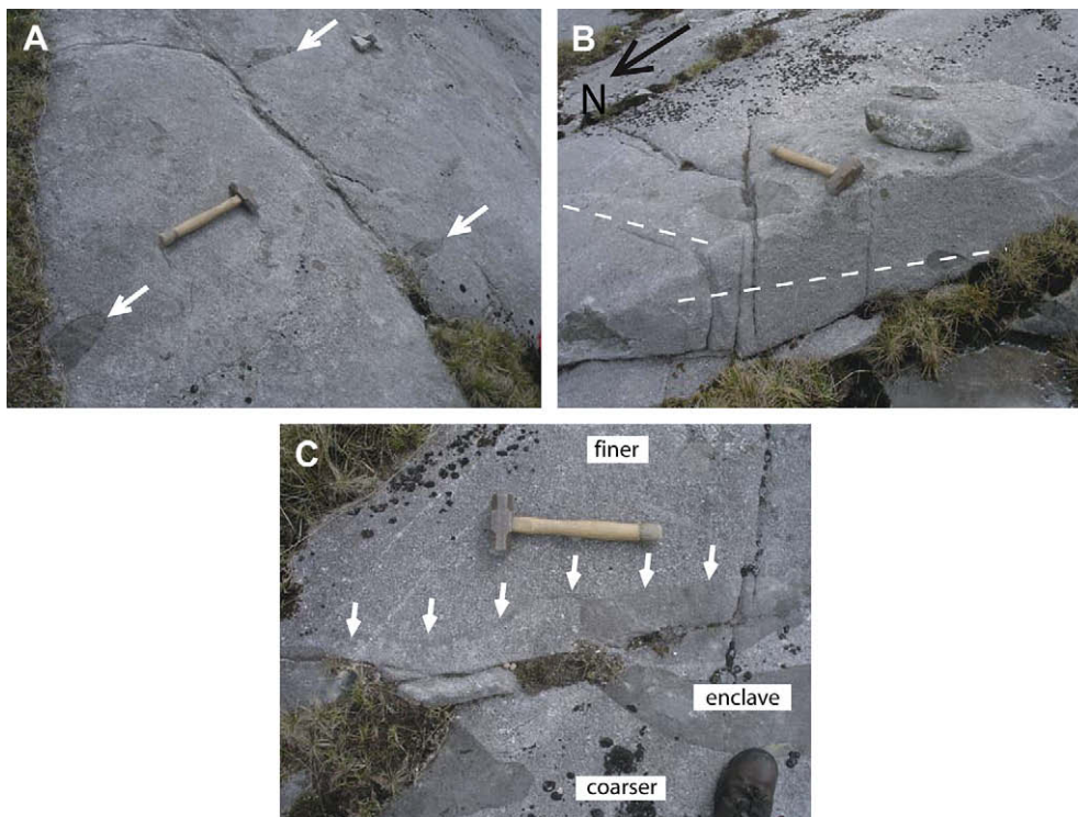
Fig. 7. (A) Field photograph of an outcrop of microgranite from the Crovehy Sheet showing enclaves of a more biotite rich microgranite (highlighted with white arrows) elongated roughly east–west (parallel with the hammer). (B) Field photograph of an outcrop of microgranite (roughly the same locality as A). Enclaves in this outcrop are flattened in a subhorizontal plane and elongated roughly east–west (parallel with the hammer). (C) Field photograph of microgranite (same locality) showing an internal contact (marked by white arrows) between a slightly coarser microgranite (pale) and a finer microgranite (darker). An enclave in the paler microgranite is truncated by the darker microgranite. This contact trends roughly east–west.
