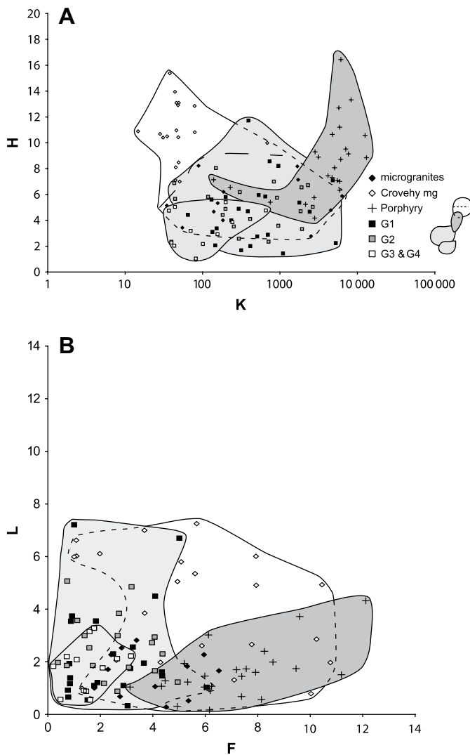
Fig. 10. (A) H plotted against K for all samples from the Rosses Complex. Data for each unit has been outlined and background shaded in varying white to grey for clarity. (B) L/F plot for all samples from the Rosses Complex, symbols and outlines are as in part A.
