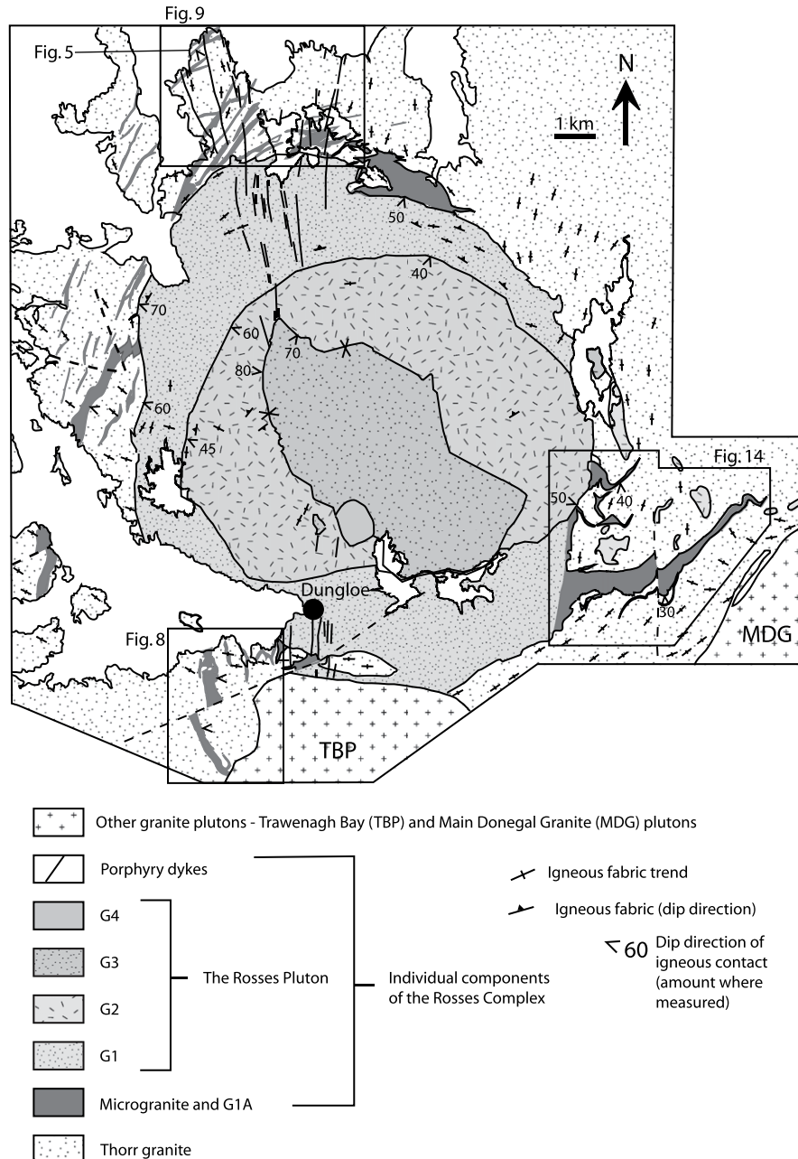
Fig. 2. The geology of the Rosses area modified after Pitcher (1953a). The metasedimentary xenoliths of the Thorr Pluton are omitted.
