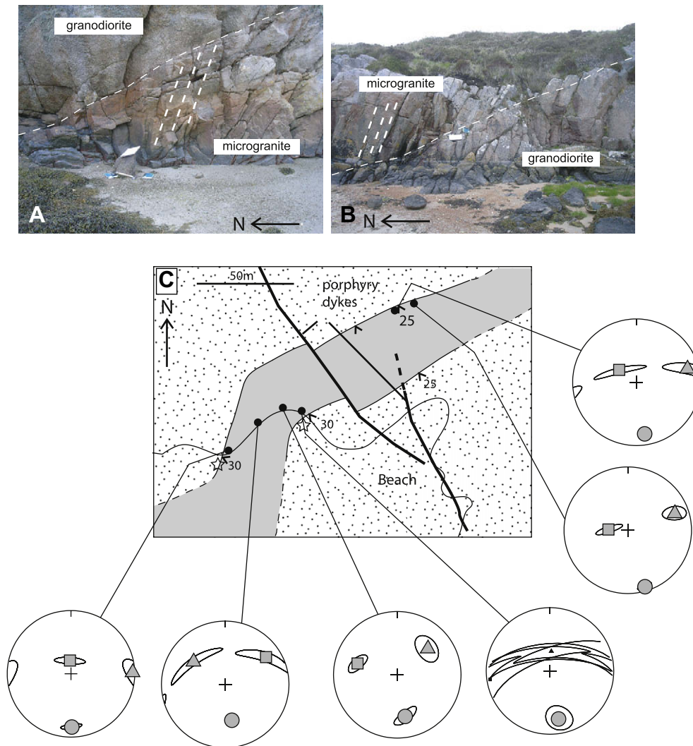
Fig. 13. (A) Field photograph showing the upper contact of a microgranite sheet. (B) Field photograph showing the lower contact of the same sheet with the apparent dip of visible fabric (feldspar alignment) indicated. (C) Sketch map of this locality (microgranite is grey). The dip of contacts is also shown. Indicated are AMS sample points and the orientation data from these samples plotted stereographically (axis labelled as in Fig. 12). Note the dextral offset of microgranite across an NE striking porphyry dyke.
