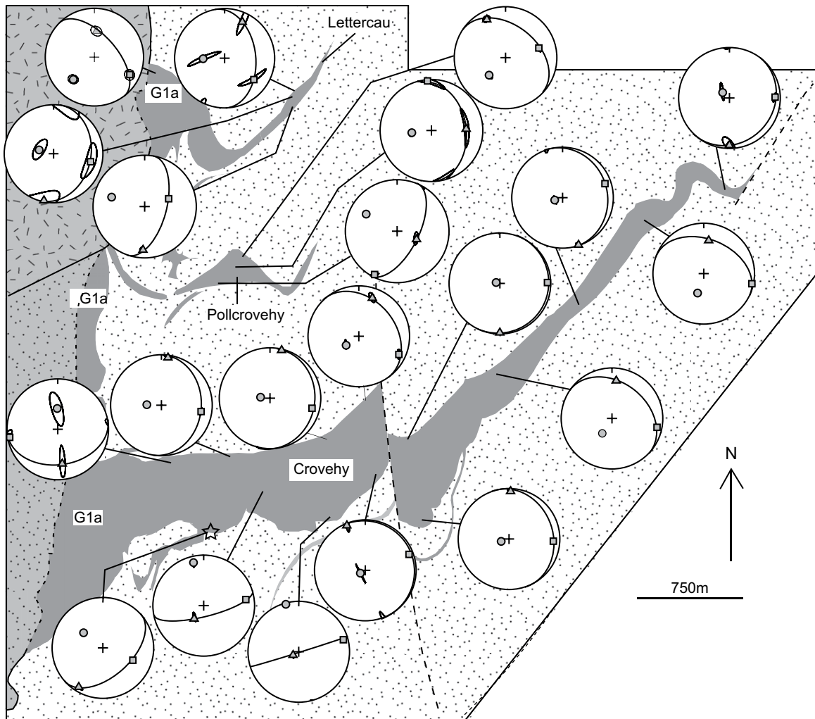
Fig. 14. Sketch map of the microgranite sheets in the east. Lithology fills are as in Fig. 1. AMS data is plotted stereographically; symbols are as in Fig. 12. Note the generally subhorizontal dip of the magnetic foliation and the east-west gently plunging lineation. Star indicates the location of the Supplementary map.
