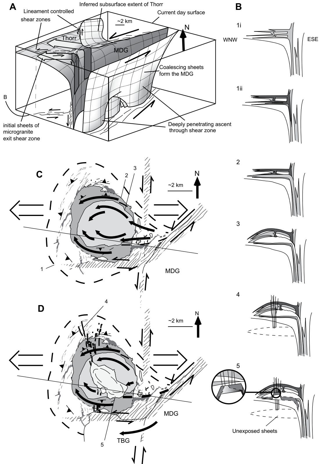
Fig. 18. Final model. (A) 3D box diagram showing a portion of the floor of the Thorr Plutons and a large part of the Main Donegal Granite (MDG) at the time of the initial microgranite sheet emplacement extending vertically from the present day surface to ~6–8 km. (B) Sketch cross section roughly corresponding to the SE side of the box of part A (and to roughly the same scale), showing the emplacement of each member of the Rosses Complex. 1 i and ii – microgranite sheets, 2 – G1, 3 – G2, 4 – porphyry dykes, 5 – G3 (inset shows G4). (C) Summary of map based on present day exposure level of the main forceful phase (parts B1–B3). Note that the Trawenagh Bay Granite to the south has not yet been emplaced. Large open arrows show the regional east-west tensional tectonic strain. Smaller shear couple arrows show the main shear zones (after Stevenson et al., in press). Thick dashed line represents the postulated (unexposed today) extent of the microgranite sheets and G2. Strike bars with a dip barb demonstrate how the microgranite sheets and fabrics in G1 dip away from the forceful and substantive G2 dome. Thick arrows represent the interpreted magma flow pathways from AMS data. The line of section for part B is shown. (D) Summary of map based on present day exposure level of the main passive phase (parts B4–B5). Note that the Trawenagh Bay Granite to the south has now been emplaced sometime just after the porphyry dykes (B4). All other arrows and symbols are as on part C.
