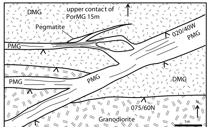
Fig. 5. Sketch map of the contact relations of a dark microgranite sheet (DMG) cut by a pale microgranite sheet (PMG) (see Fig. 2 for location). Both of these intrude Thorr granodiorite. Thin lines represent faint banding in the PMG. The offset of the DMG contact across the PMG sheets is in a reverse sense. The strike/dip and dip direction is noted for some contacts.
