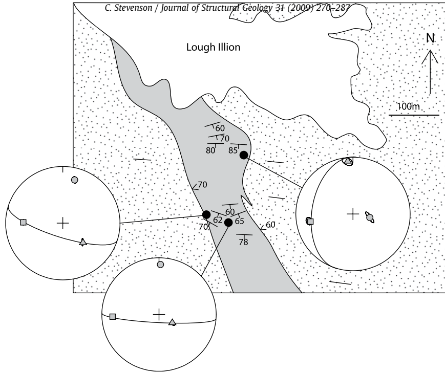
Fig. 15. Sketch map of a microgranite sheet (grey) in the southwest, with visible fabric orientations marked with strike and dip bars and stereographic plots of AMS orientation data. Observed fabric trace in the Thorri granodiorite is marked with a dash. Note the steep magnetic foliations roughly parallel to visible fabrics, presumably tectonic related, and gently dipping fabric from one AMS station parallel to the margin, possibly primary magmatic.
