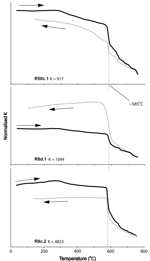
Fig. 11. Susceptibility with varying temperature for three representative samples from the Rosses Complex. On each plot, the heating curve is in black and the cooling curve in grey. The susceptibility ( K ) is shown for each sample. Heating curves indicate the Curie temperature of magnetite ( \sim 585^\circ\text{C} ).
